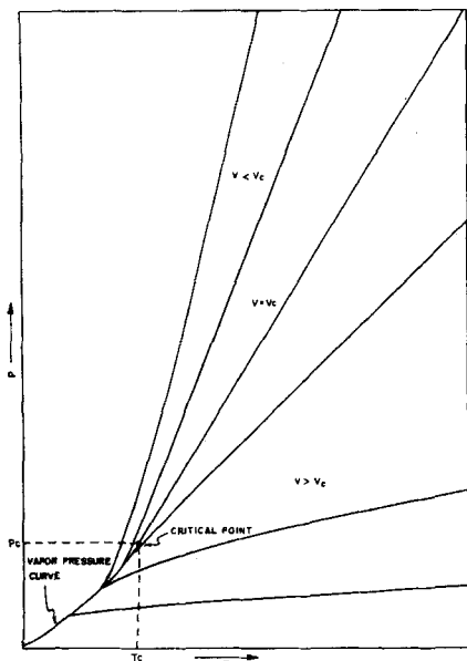
FIG. 6. PRESSURE-TEMPERATURE DIAGRAM.
