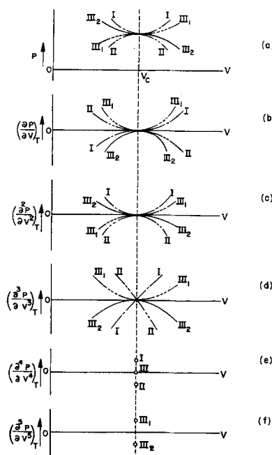
FIG. 4. PRESSURE-VOLUME DERIVATIVES WHEN \left(\frac{\partial^3 P}{\partial V^3}\right)_{T_c} = 0 AT CRITICAL POINT. [IT IS TAKEN FOR GRANTED THAT \left(\frac{\partial P}{\partial V}\right)_{T_c} = 0 , AND \left(\frac{\partial^2 P}{\partial V^2}\right)_{T_c} = 0 AT CRITICAL POINT.]
